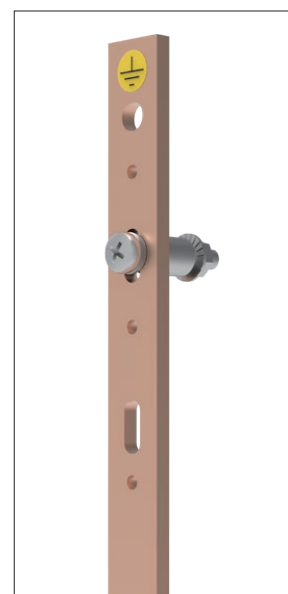
Vertical earthing bar, fastened to C-profiles
