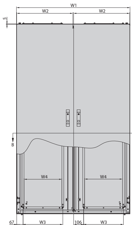
Front view (cabinet with double-leaf door)
