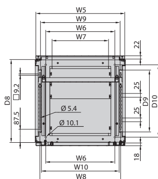
C-C section
