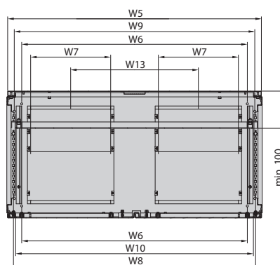
B-B section
