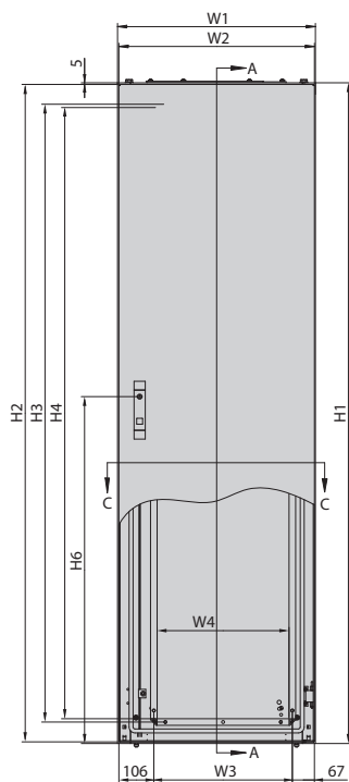
Front view (cabinet with single-leaf door)
